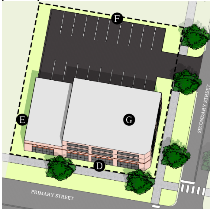
(b) BUILDING PLACEMENT
