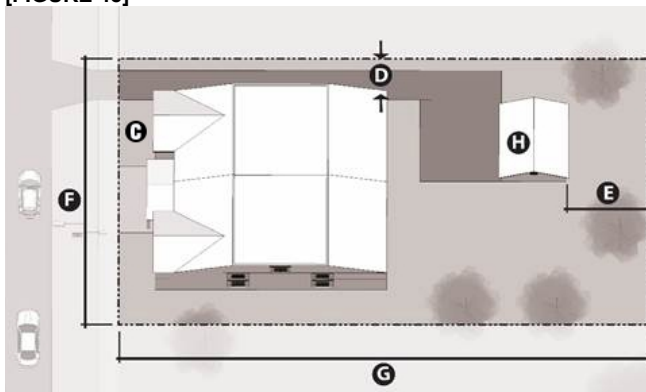
(b) BUILDING PLACEMENT
